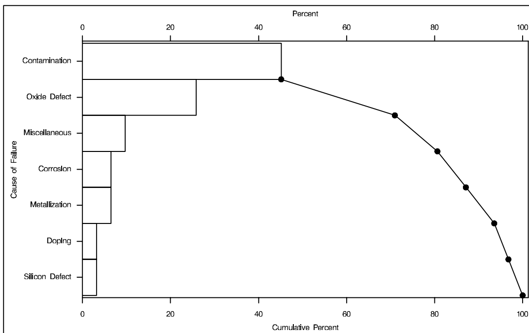
Figure 27.1. Pareto Chart for IC Failures in the Data Set FAILURE1
